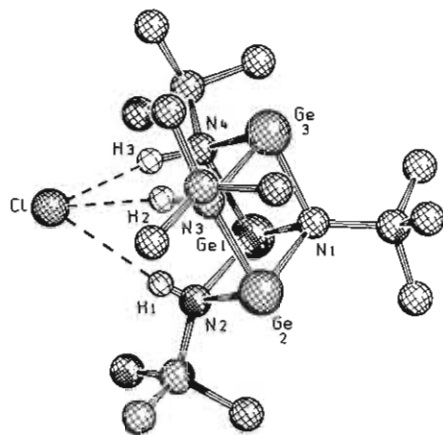
Figure 1. Graphic representation of \text{Ge}_3(\text{N-}t\text{-Bu})_4\text{H}_3\text{Cl} ( 1 ) based on the single-crystal X-ray structure determination.
